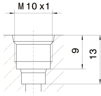
Fig. 4: Profiled bore for M 10 x 1 thread
