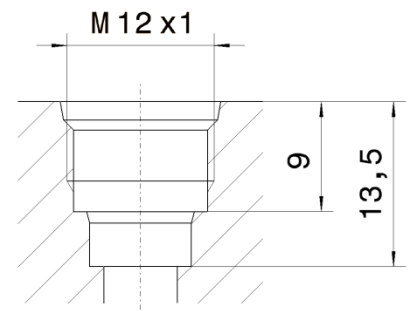
Fig. 5: Profiled bore for M 12 x 1 thread
